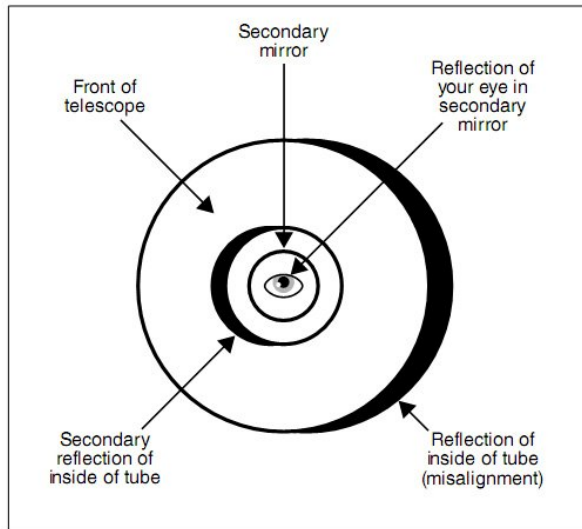
Figure 6-2 – Out of collimation (alignment) optics as seen through the rear of the telescope.
