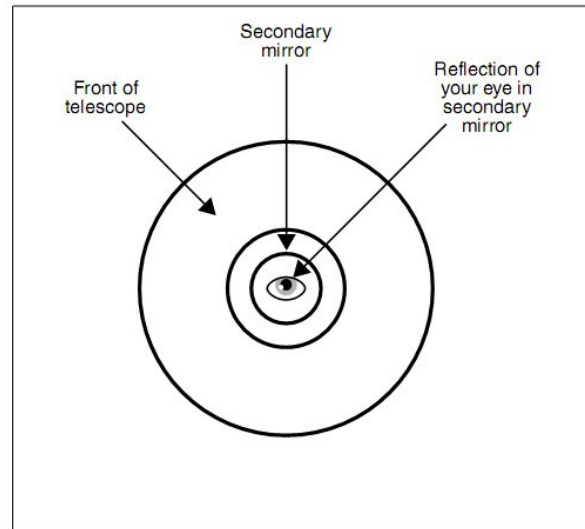
Figure 6-3 – Collimated (aligned) optics as seen through the rear of the telescope.
