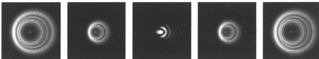
Figure 6-1 -- Even though the star pattern appears the same on both sides of focus, they are asymmetric. The dark obstruction is skewed off to the left side of the diffraction pattern indicating poor collimation.
